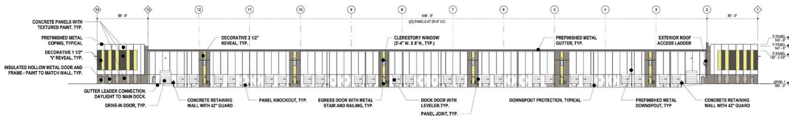
SOUTH ELEVATION 1" = 30'0"
